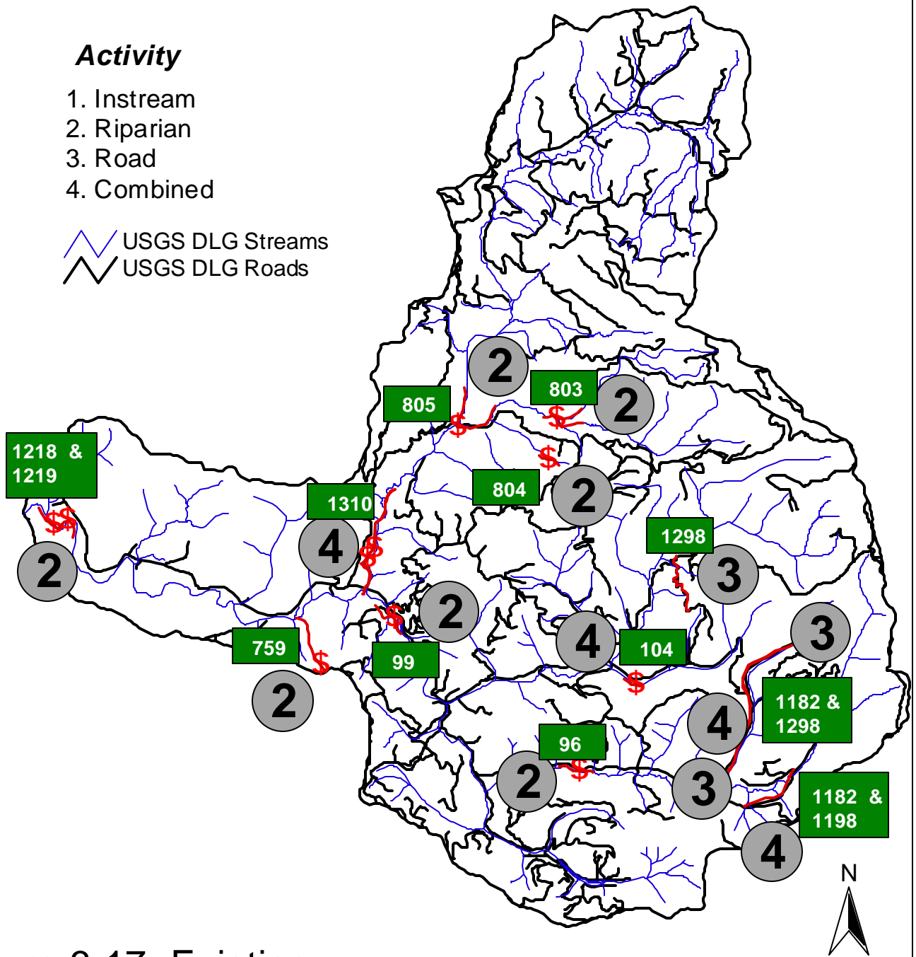
Figure 3.17. Existing restoration sites in the Rock Creek watershed. Boxed numbers correspond to individual projects (see text).
