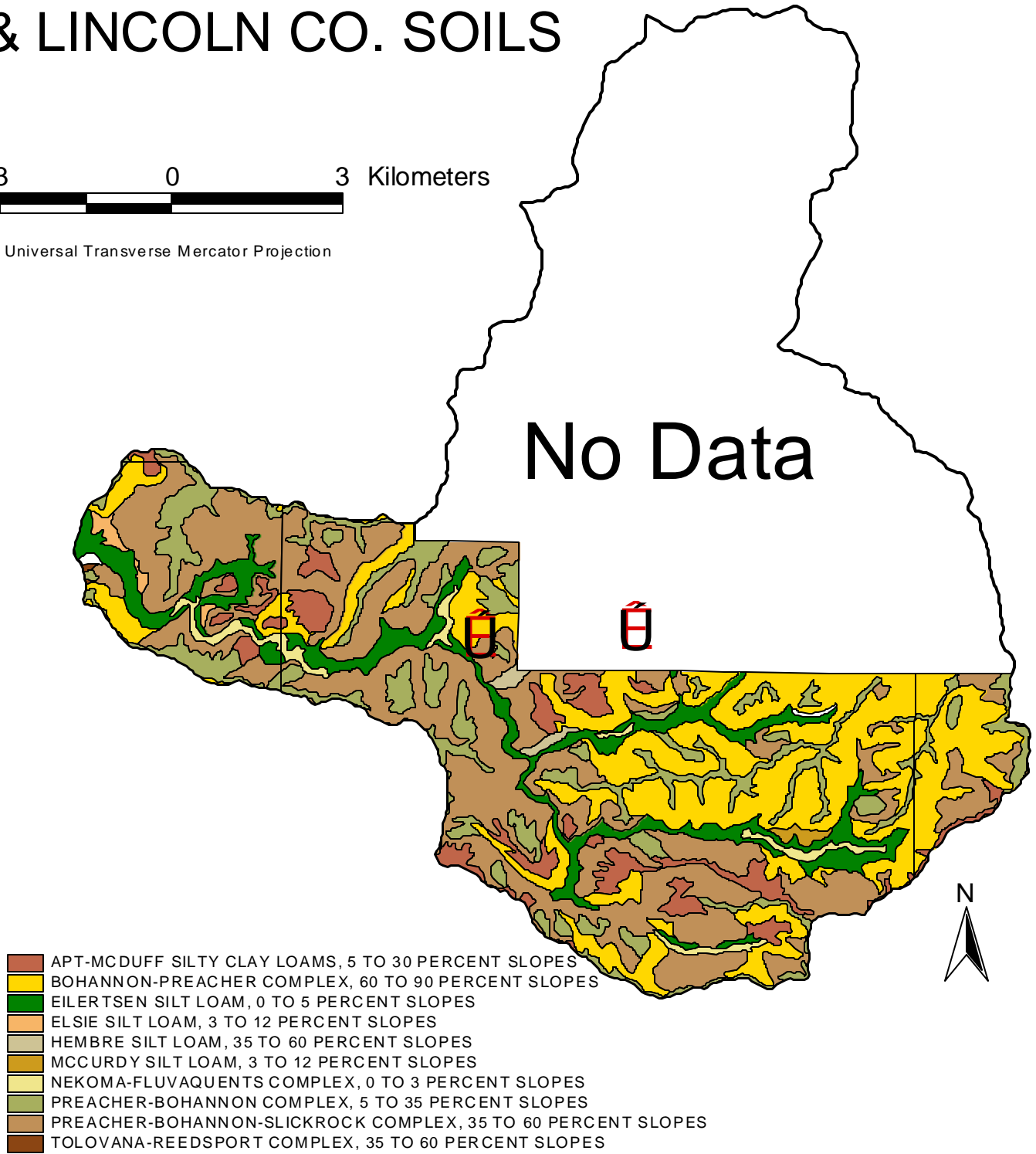
Figure 3.5. Mapped landslides and Lincoln County soils.
