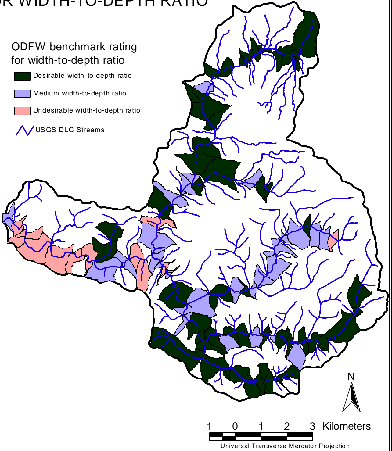
Figure 5.4. ODFW benchmark rating for width-to-depth ratio, by catchment (from AHI data).
