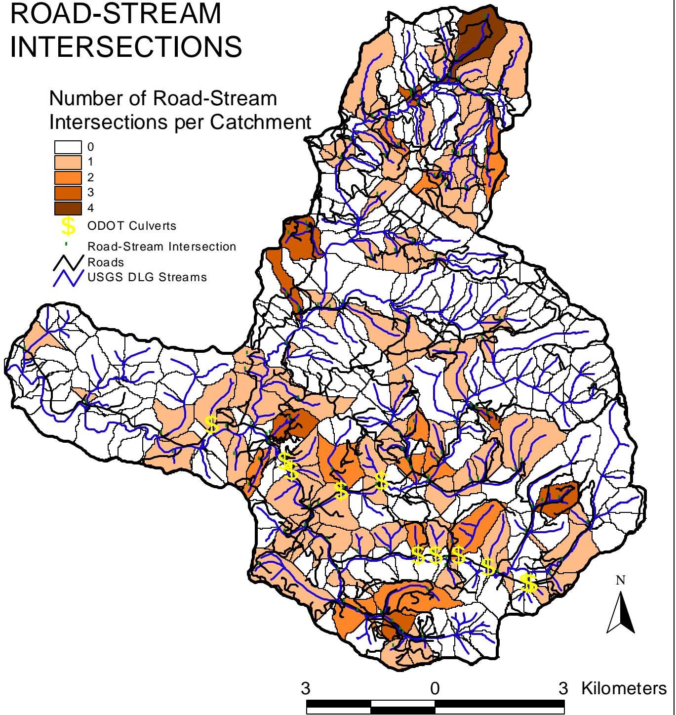
Figure 5.11. ODOT culverts, potential stream crossings, and potential road-stream intersection density.
