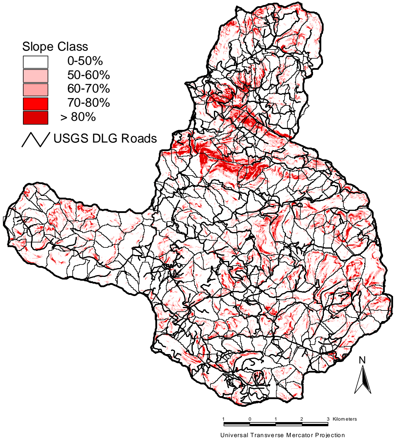
Figure 6.1. Slope classes derived from 10 M DEMs.
